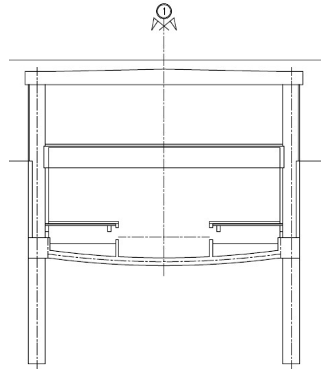
Figure 8. Typical cross-section of a cut&cover station.
