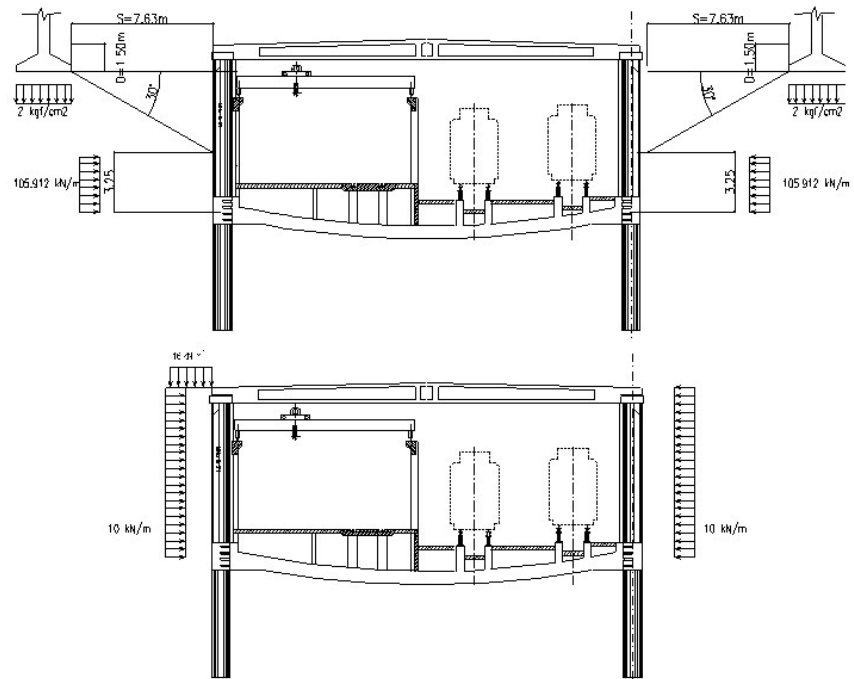
Figure 13. Structural model for designing Line D Maintenance Facility (reproduced with permission from the calculation notes of the project).
