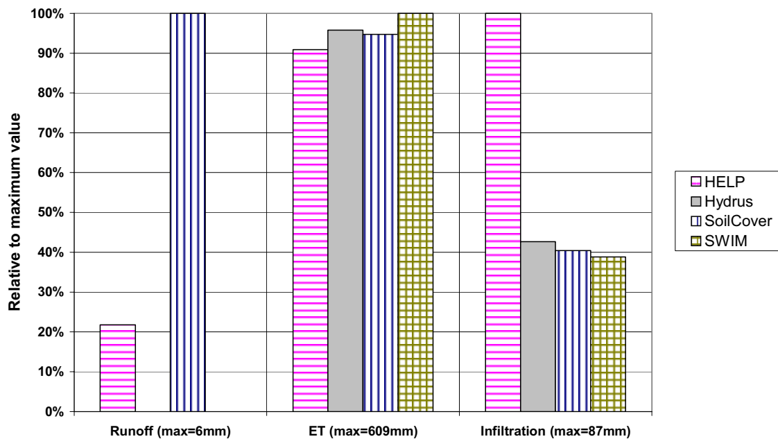
FIG 4 - Water balance comparison, calibration case.
