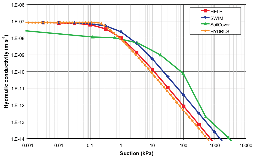
FIG 2 - Fitted unsaturated hydraulic conductivity functions for weathered waste rock.
