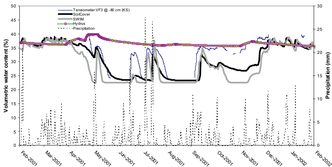
FIG 3 - Volumetric water content and precipitation vs time, modelling results and tensiometer measurements at bottom of topsoil layer.
