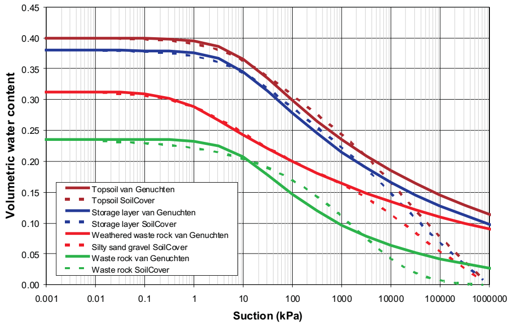
FIG 1 - Fitted soil water characteristic curves.
