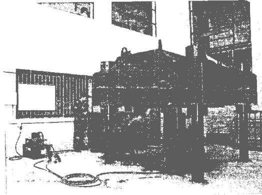
Figure 3 Triaxial equipment at IDIEM laboratory
