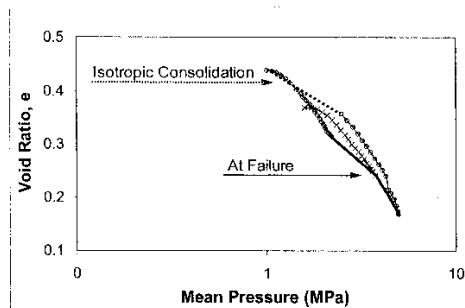
Figure 22 Voids Ratio versus Mean pressure, "truncated" PSD
