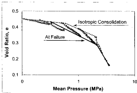
Figure 21 Voids ratio versus Mean pressure, "parallel" PSD
