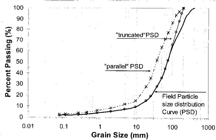
Figure 6 Particle size distributions: field sample curve, "parallel" curve and "truncated" curve
