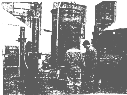
Figure 4 Assembly of a specimen in the triaxial chamber
