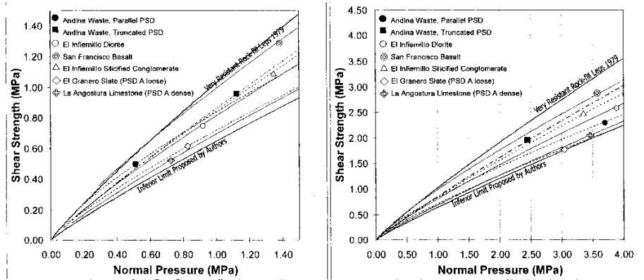
Figure 18 Andina waste shear resistance envelope and comparison with other material envelopes (as from quarry and angular)
